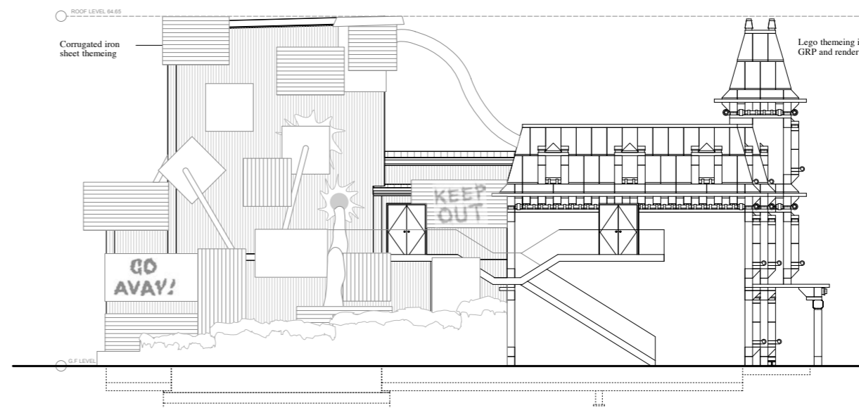
East Elevation
